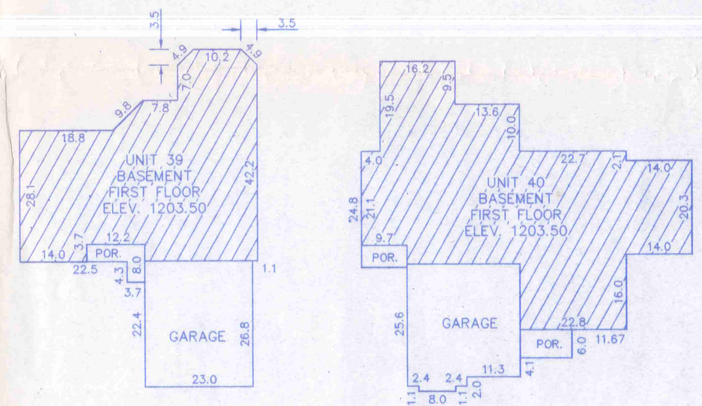
DETAIL - UNIT 39 & 40 (1" = 20')
